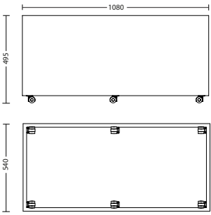
SIMPLE Duo mobile
